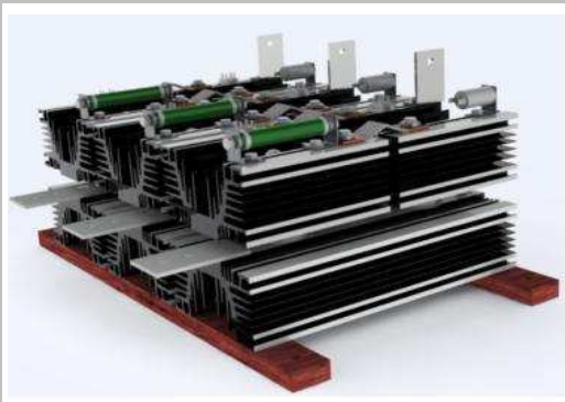
Thyristor Presspack stack
