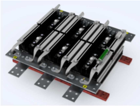
Diode Presspack stack
